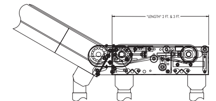
Integral Feeder
