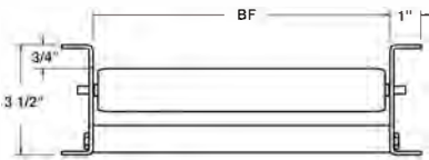
Single roller curves (12" & 18" OAW models only)
