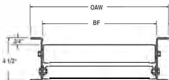
Single roller design
