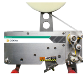
Utilizes industry leading DEKKA E tape head with an open design, making it easy to refill tape
