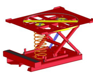
800# = 1 orange spring
