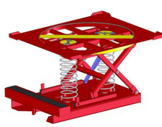
600# = 2 white springs
