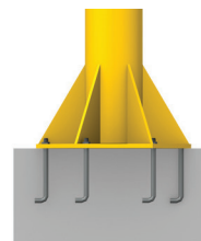
FS300 - Baseplate Mounted
